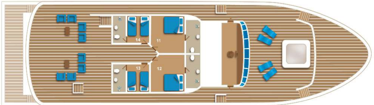
Main Deck
